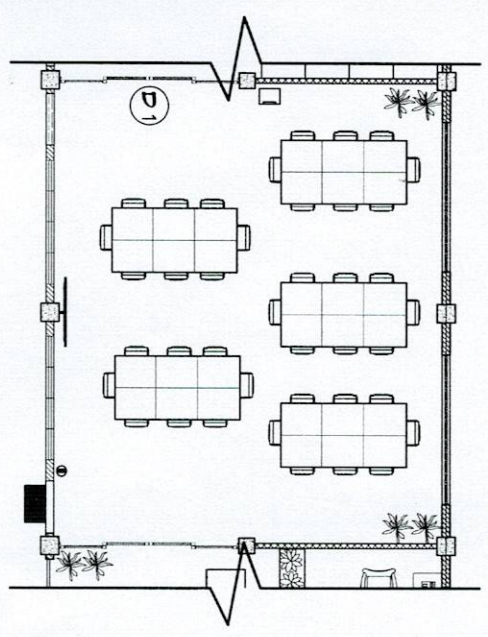
TYPICAL FLOOR PLAN SCALE 1:100 M
